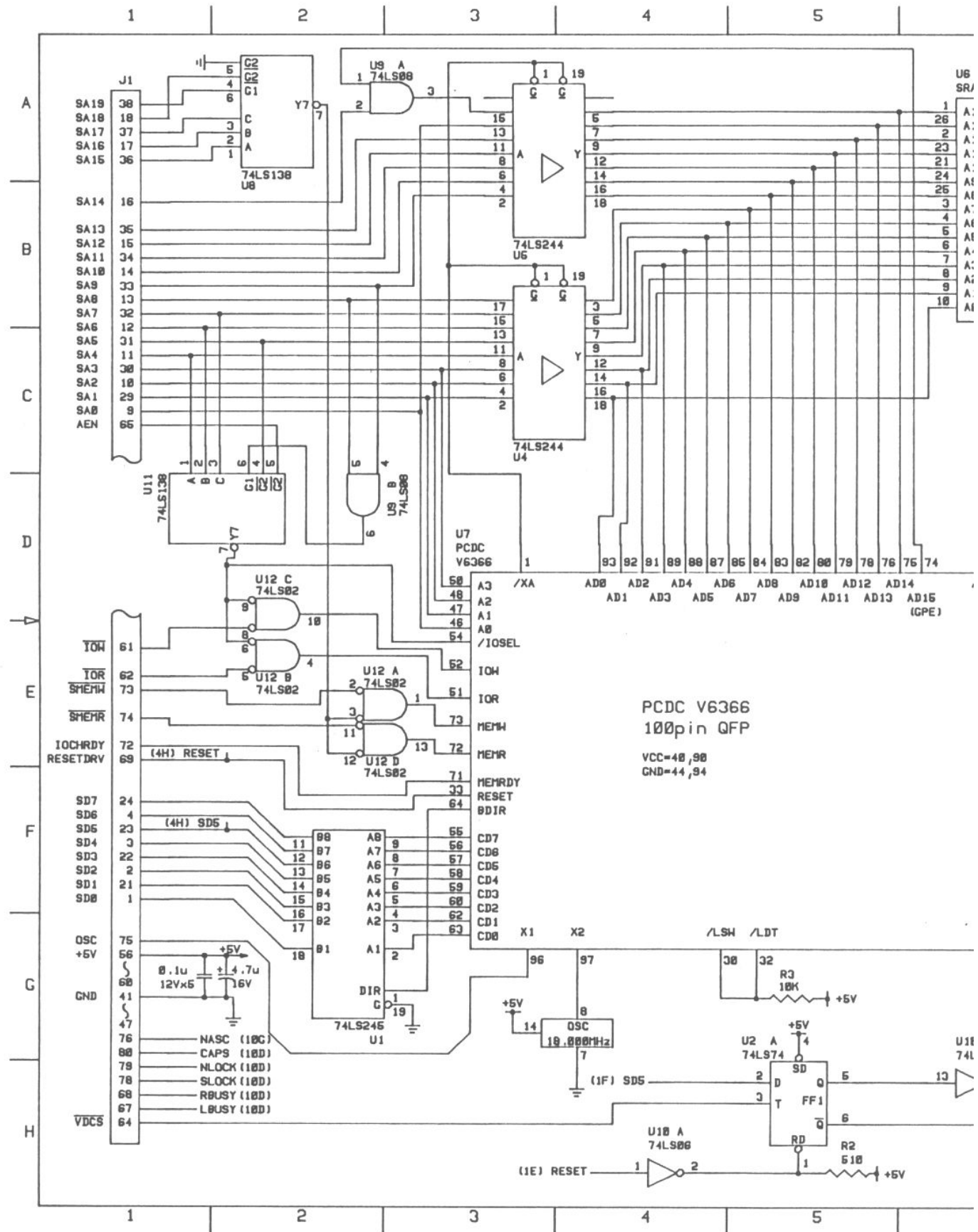
Schematic diagram 1
