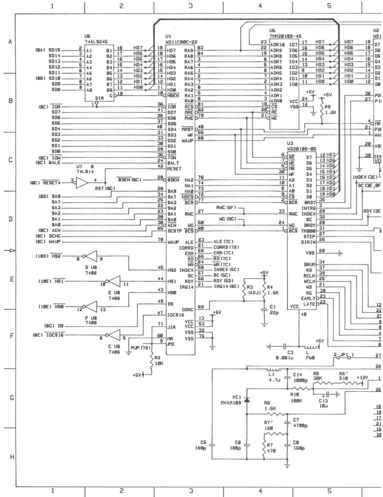
Schematic diagram 1
