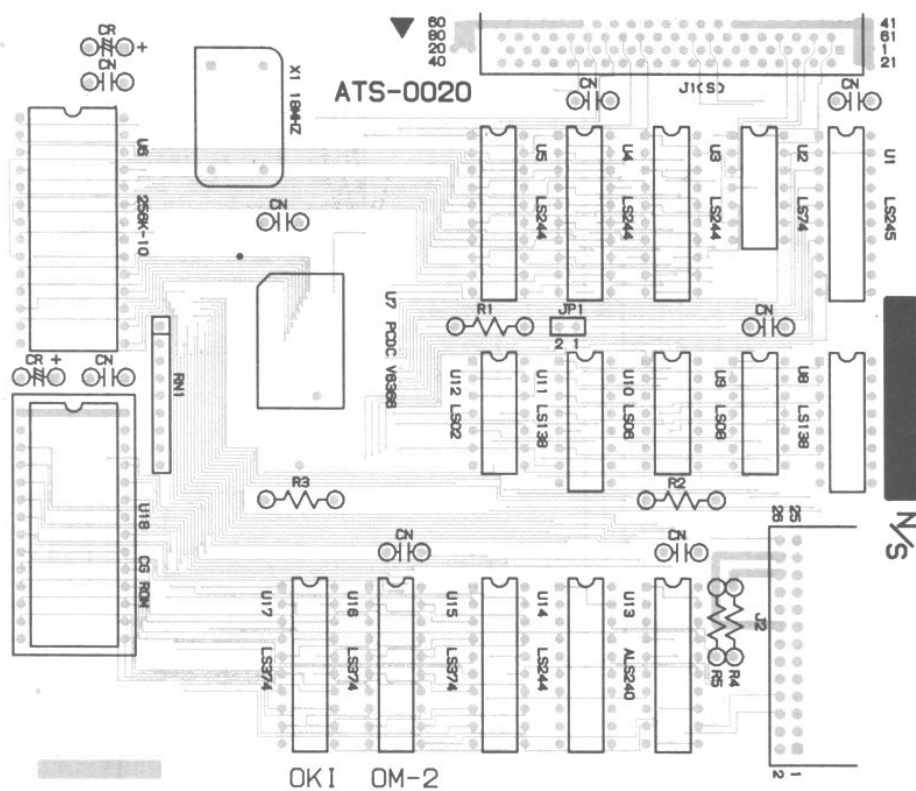
Soldering side
