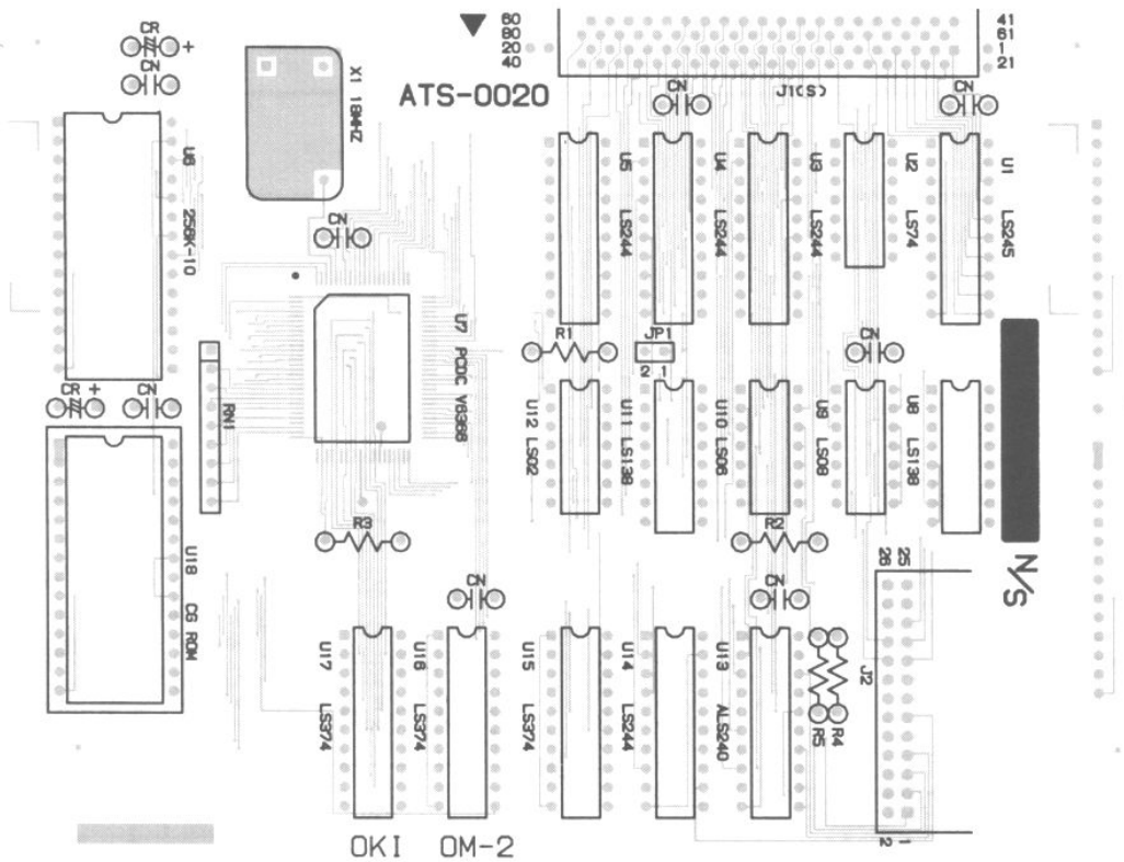
Component side
